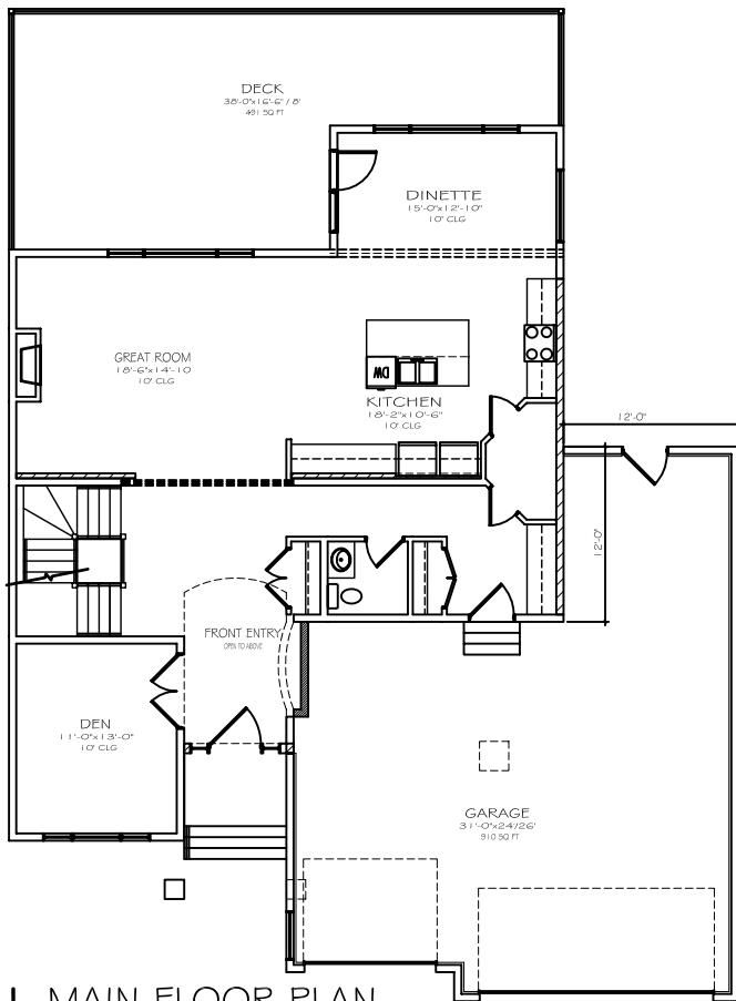
1 MAIN FLOOR PLAN 1359 SQ FT
