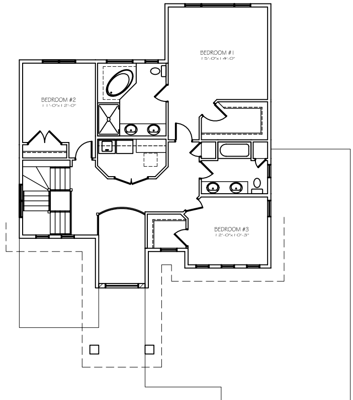
2 SECOND FLOOR PLAN 1292 SQ FT
