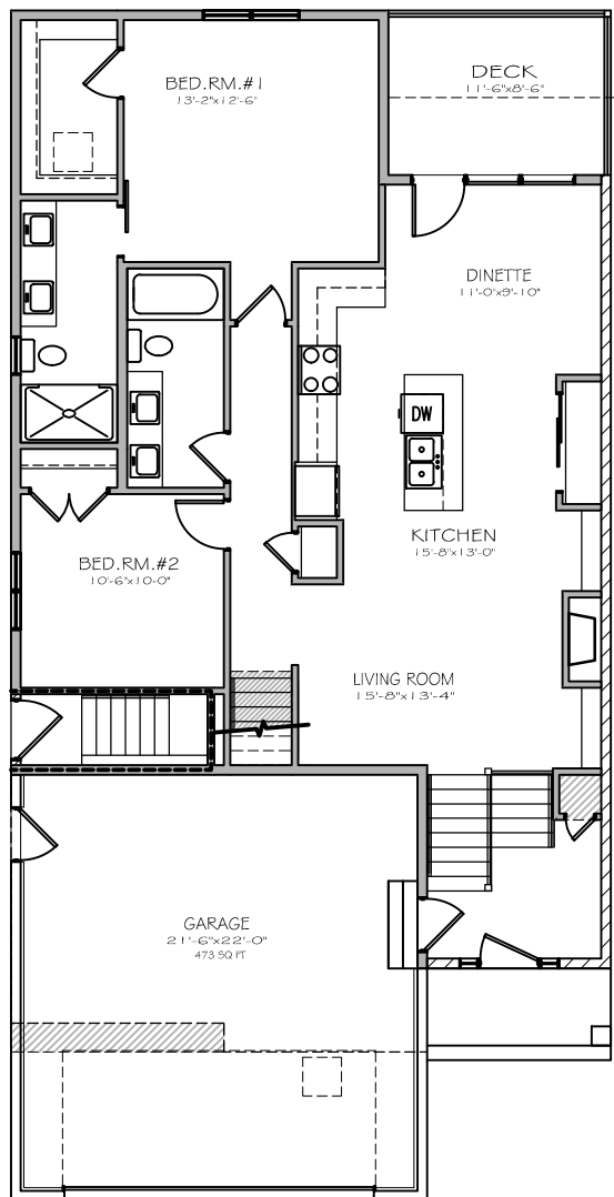
MAIN FLOOR PLAN 1180 SQ FT
