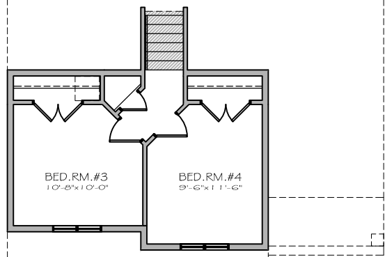
SECOND FLOOR PLAN 303 SQ FT
